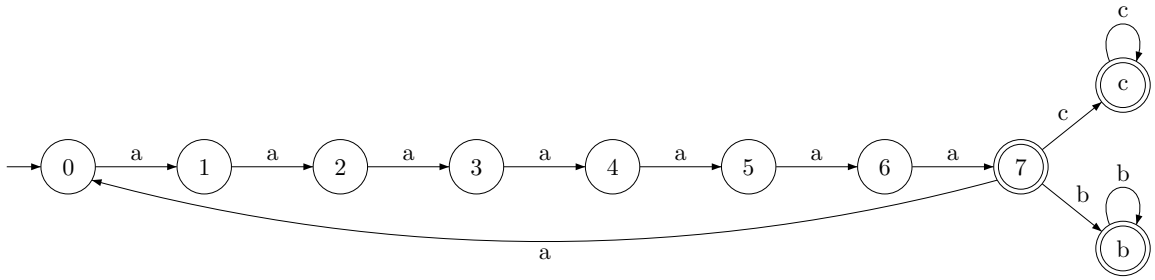
Obr. 5.3: DFA A_7 pre jazyk L_7 = a^7\{a^8\}^*\{b\}^* \cup \{c\}^*
