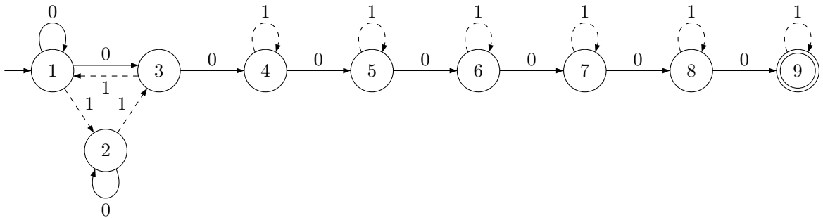
Obr. 3.1: UFA \mathcal{U}_9
