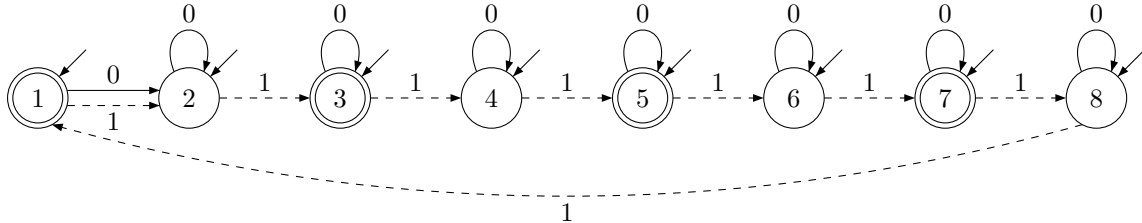
Obr. 4.1: MDFA M_8
