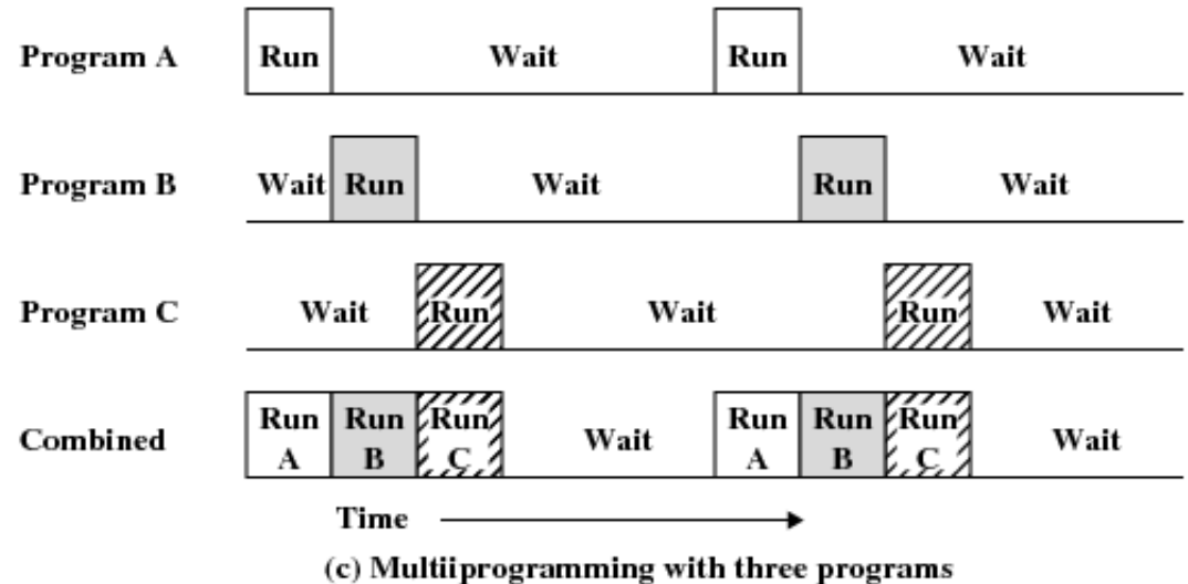
Figure 2.5 Multiprogramming Example
