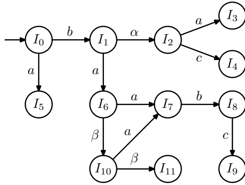
(a) Automat \mathcal{D}_G .
