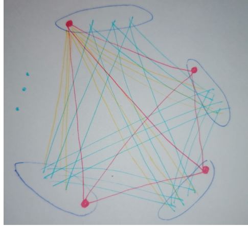
Obr. 12: T_{r-1}(n)
