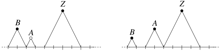
Figure 10: Two examples of Case 1
