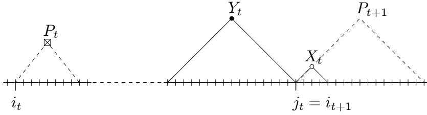
Figure 6: One iteration of the while loop in procedure DELETE.
